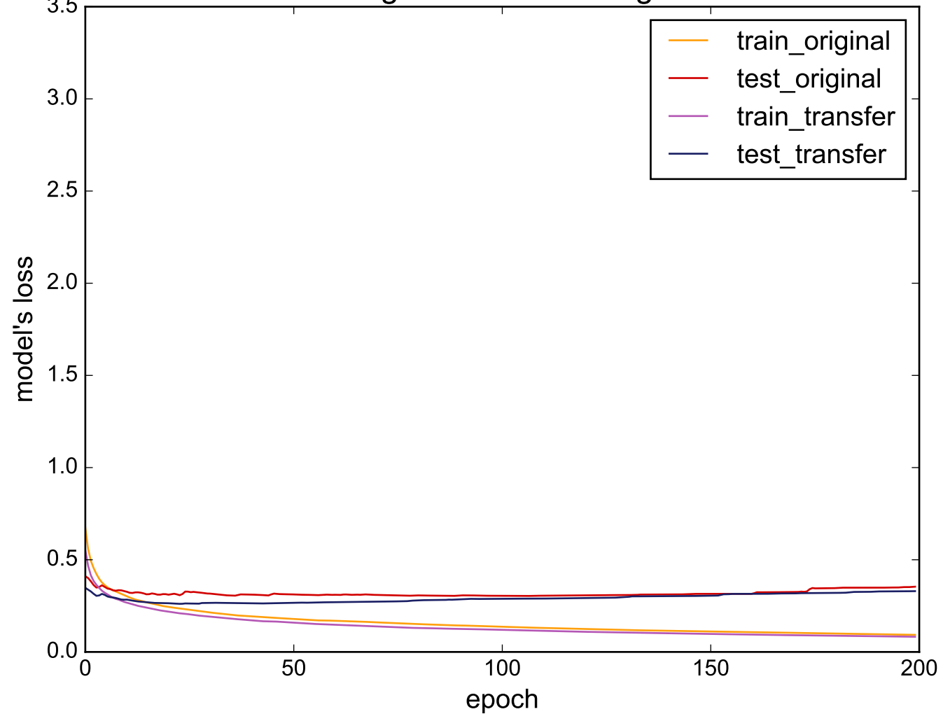
Source: ToeSegmentation2 - Target: ECG5000
