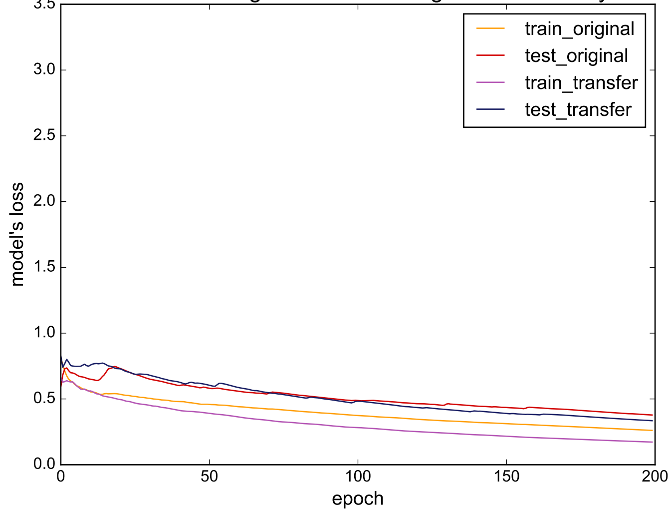
Source: ToeSegmentation2 - Target: ECGFiveDays
