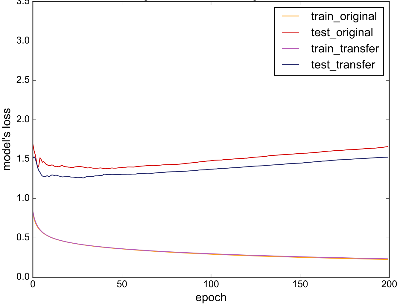
Source: ToeSegmentation2 - Target: ElectricDevices
