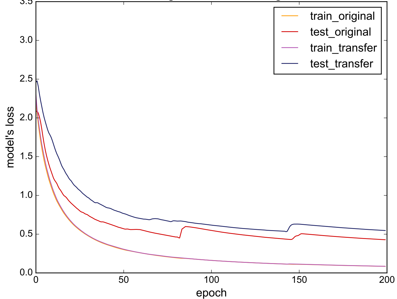
Source: ToeSegmentation2 - Target: FaceAll
