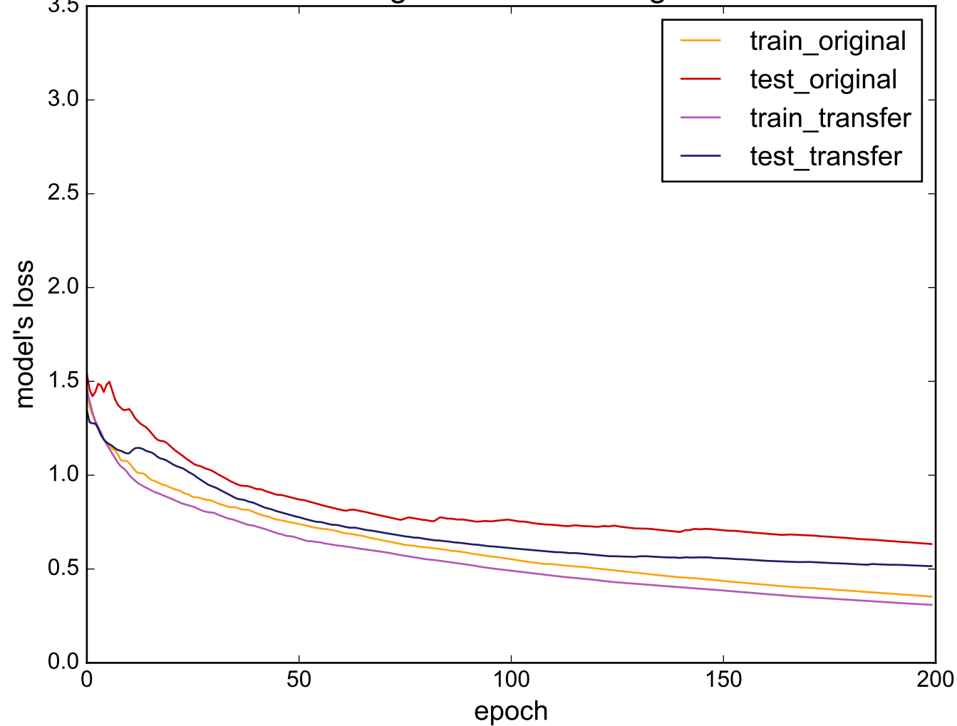
Source: ToeSegmentation2 - Target: FaceFour
