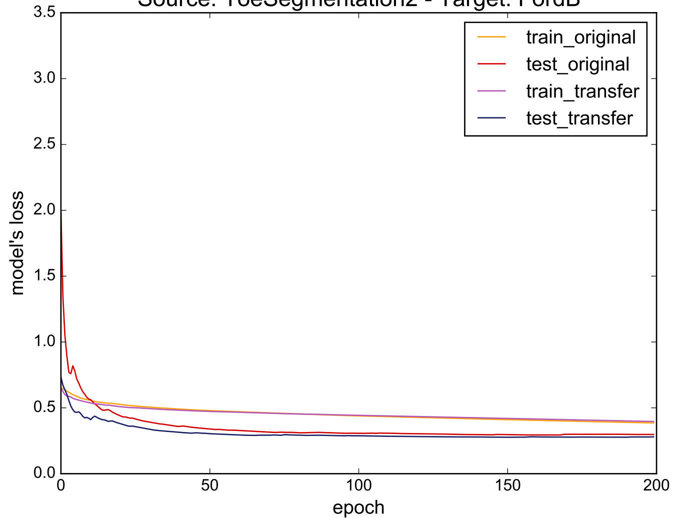
Source: ToeSegmentation2 - Target: FordB
