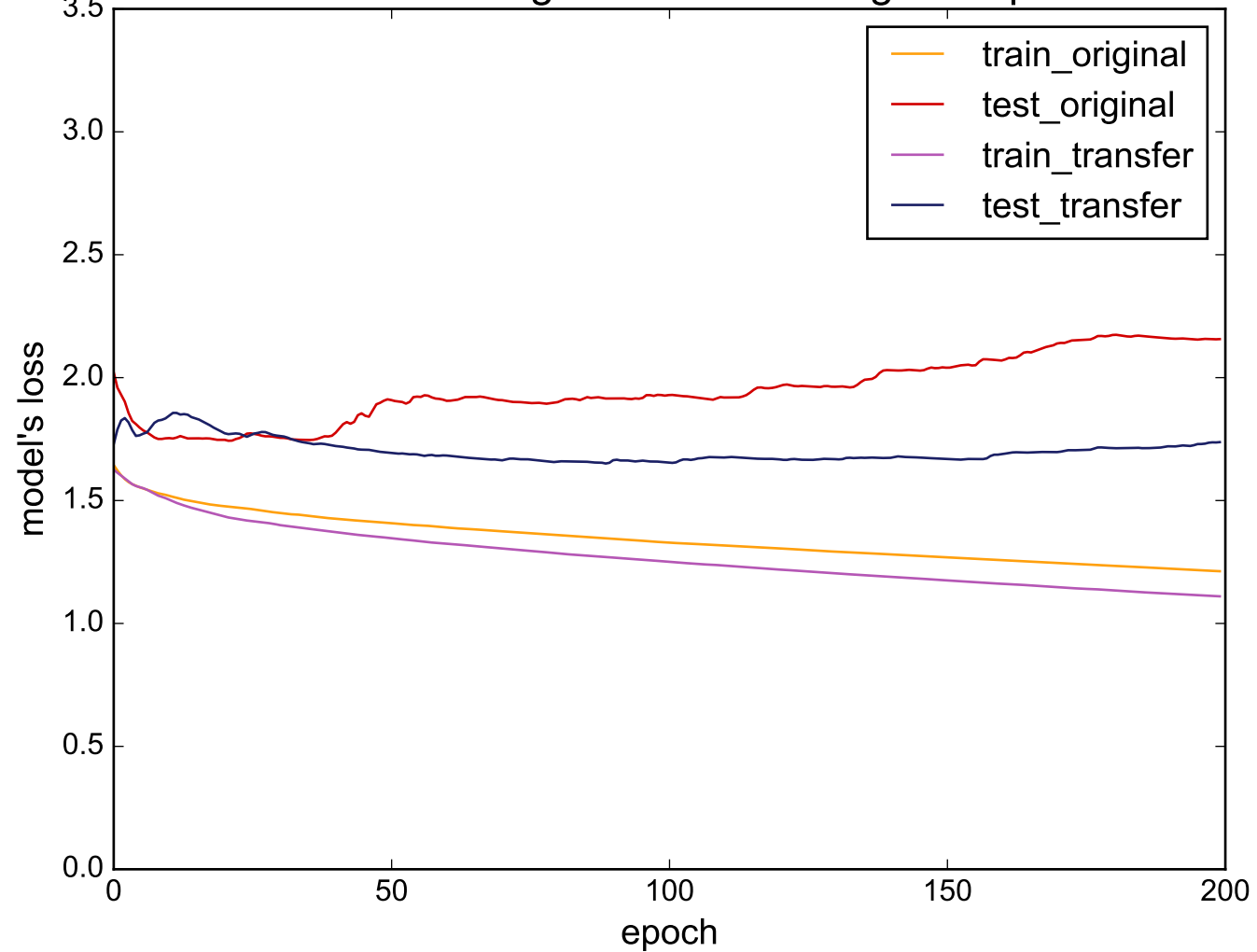
Source: ToeSegmentation2 - Target: Haptics
