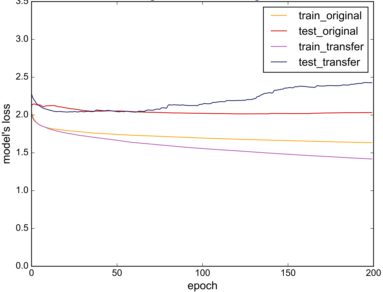
Source: ToeSegmentation2 - Target: InlineSkate
