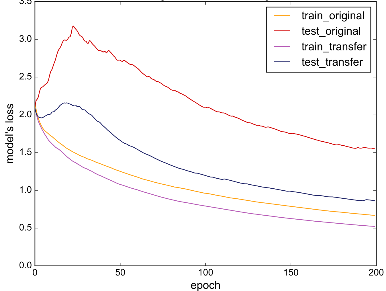
Source: ToeSegmentation2 - Target: MALLAT
