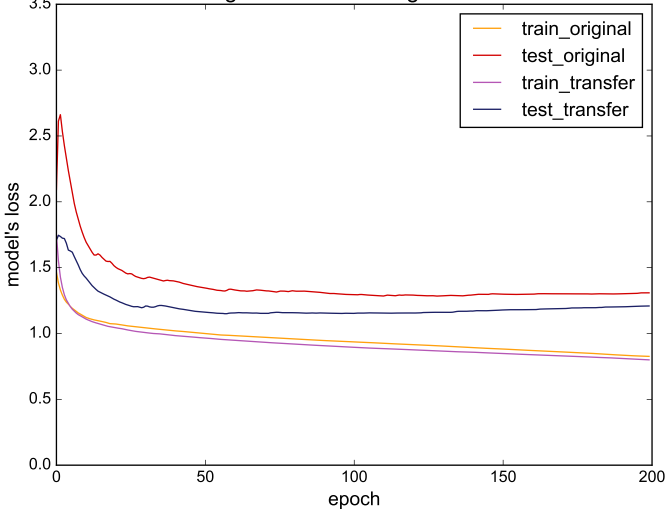
Source: ToeSegmentation2 - Target: MiddlePhalanxTW
