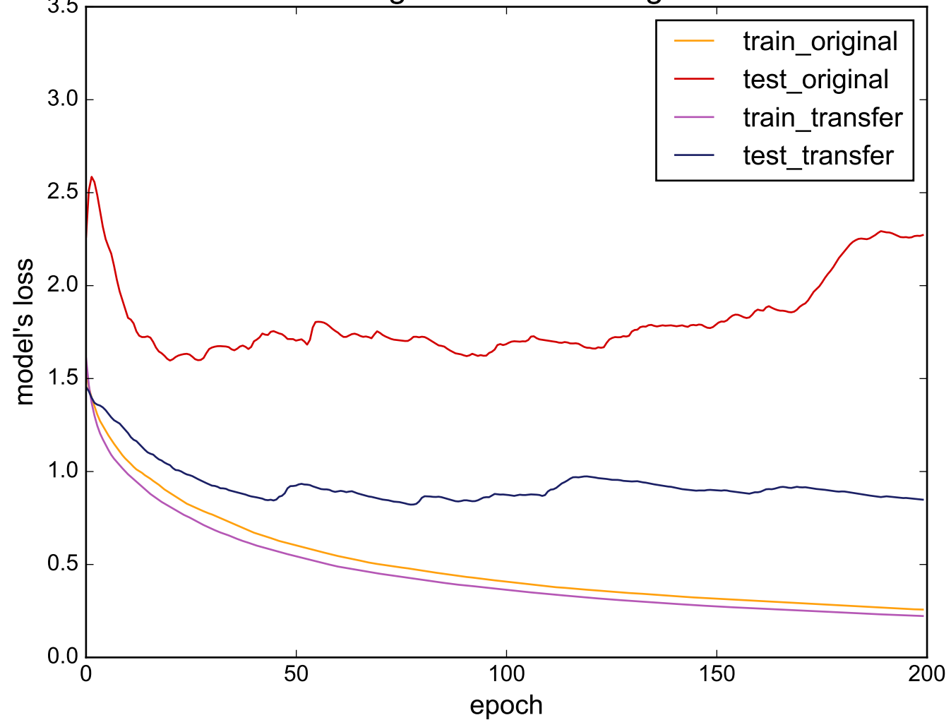
Source: ToeSegmentation2 - Target: OSULeaf
