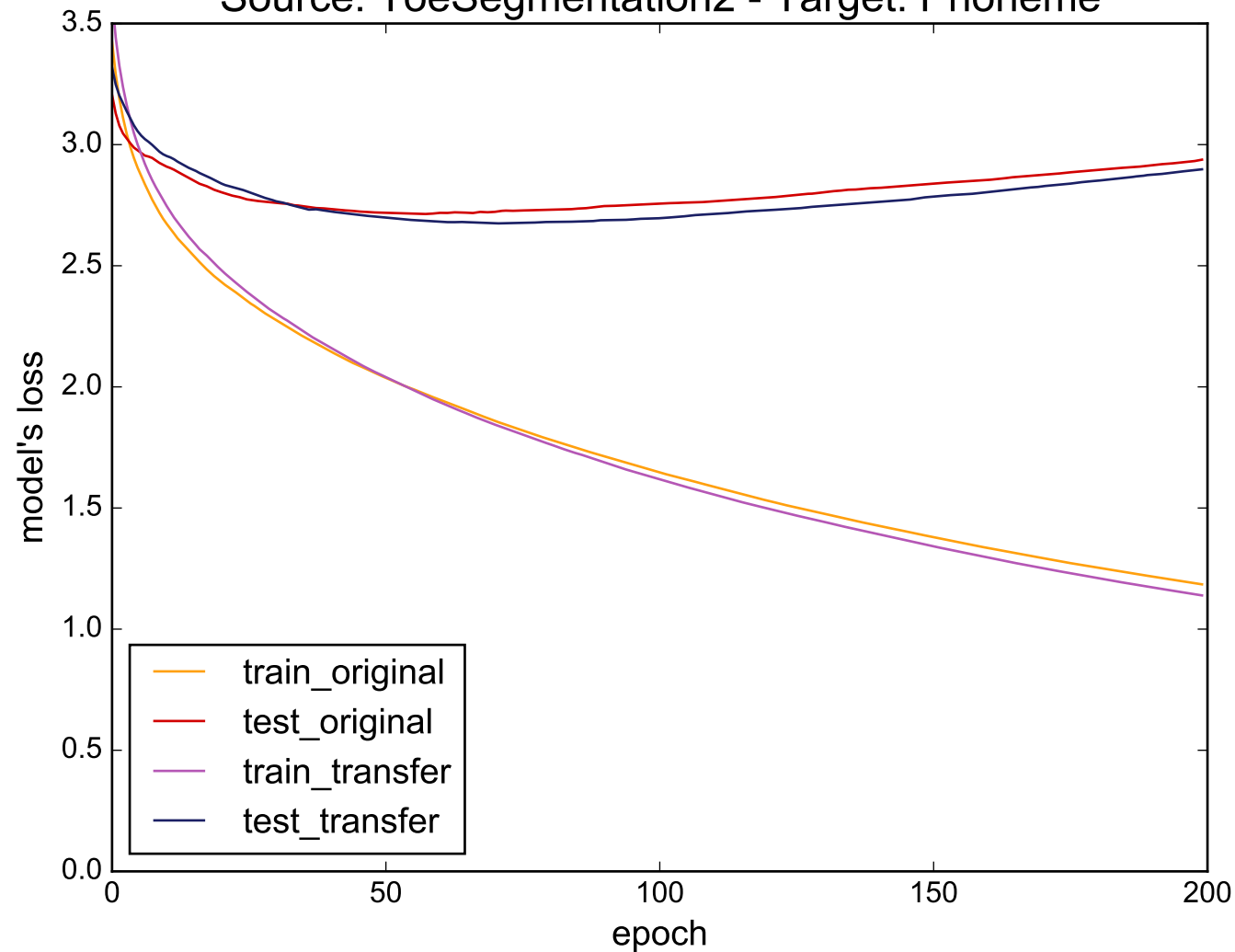
Source: ToeSegmentation2 - Target: Phoneme
