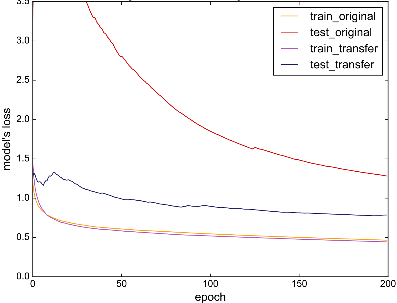
Source: ToeSegmentation2 - Target: ProximalPhalanxTW
