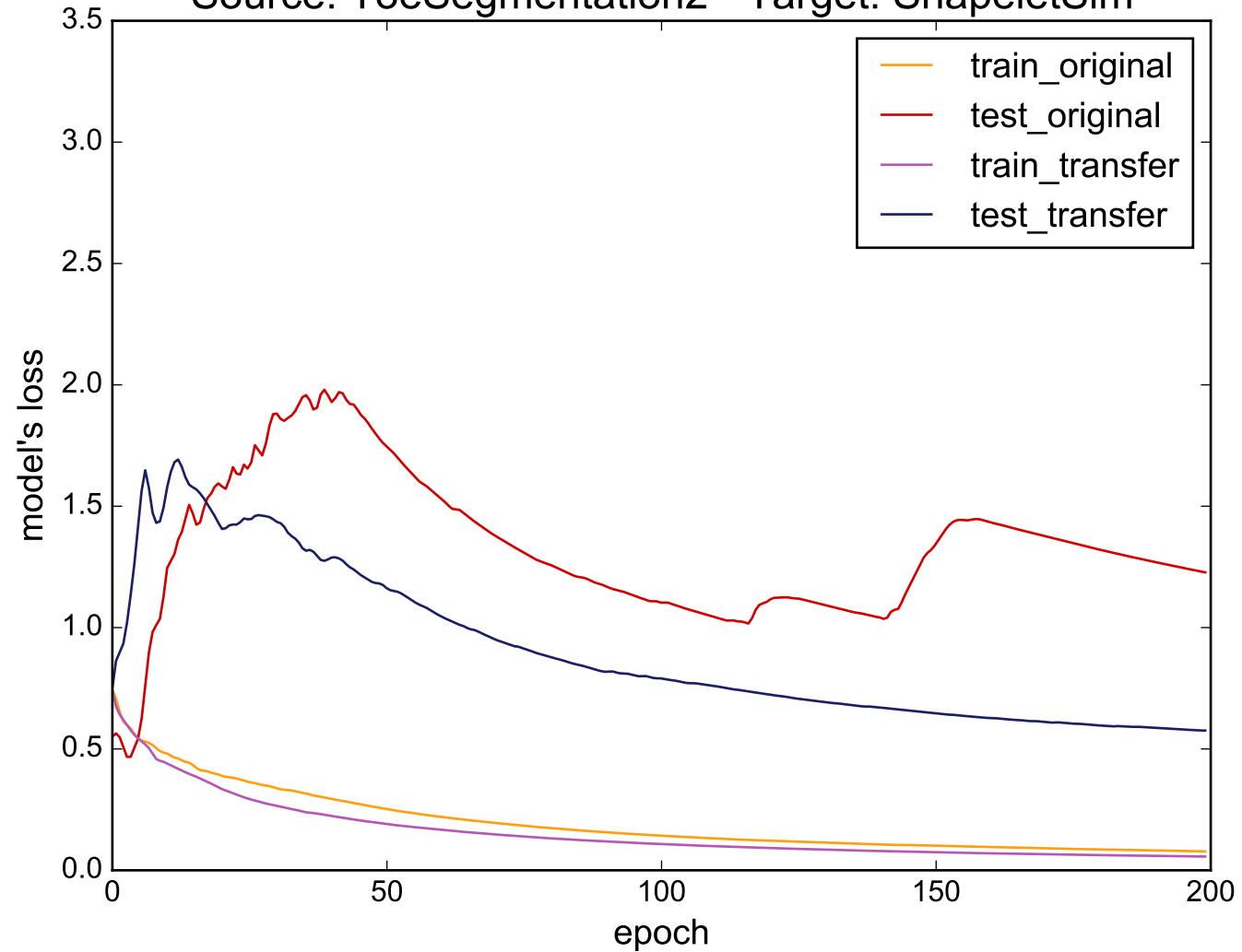
Source: ToeSegmentation2 - Target: ShapeletSim
