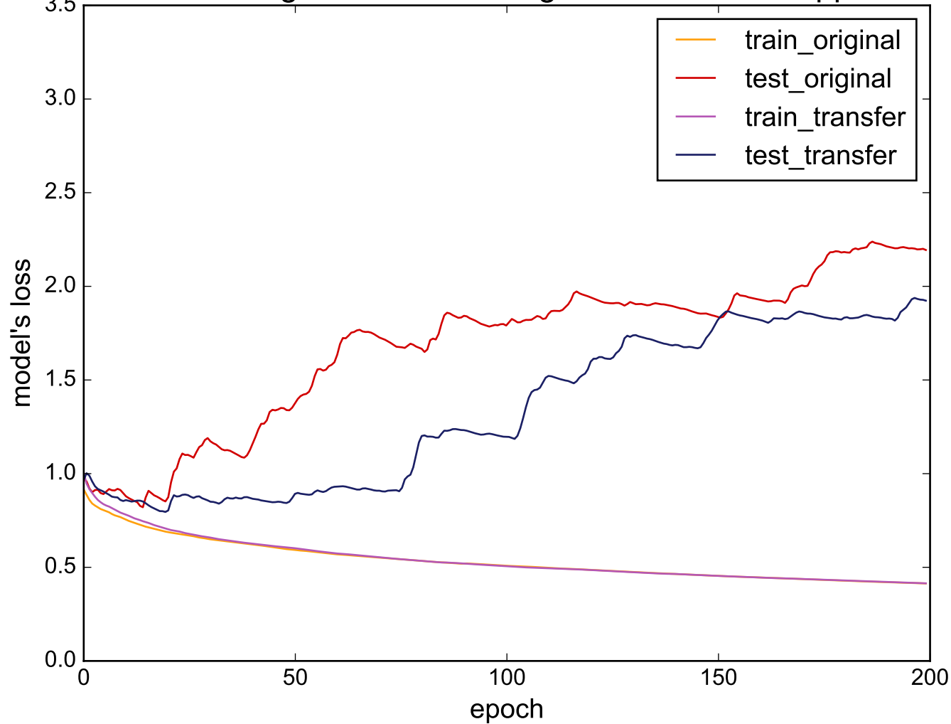
Source: ToeSegmentation2 - Target: SmallKitchenAppliances
