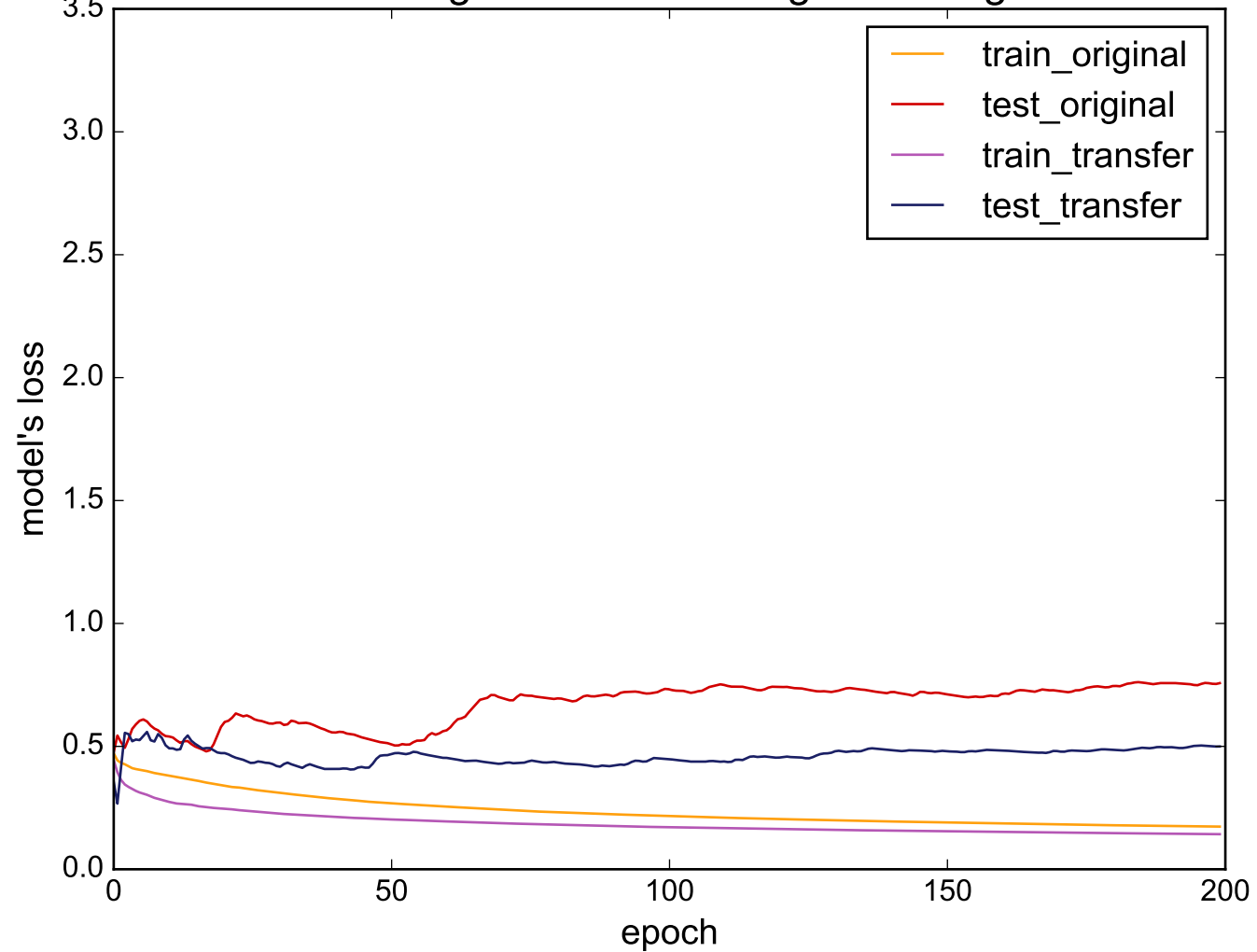
Source: ToeSegmentation2 - Target: StarLightCurves
