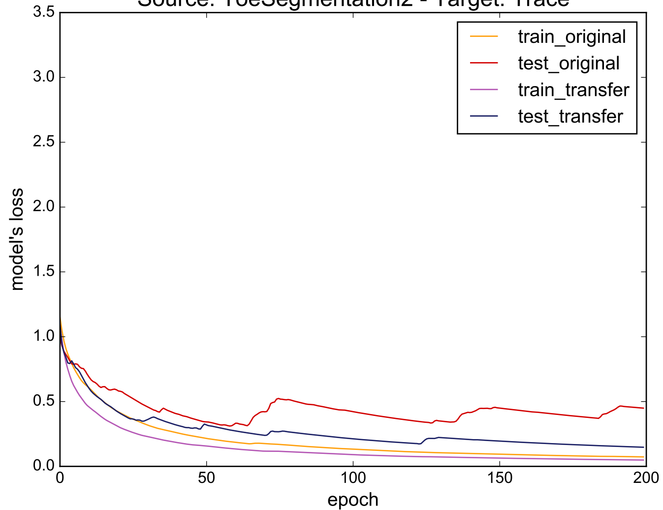
Source: ToeSegmentation2 - Target: Trace
