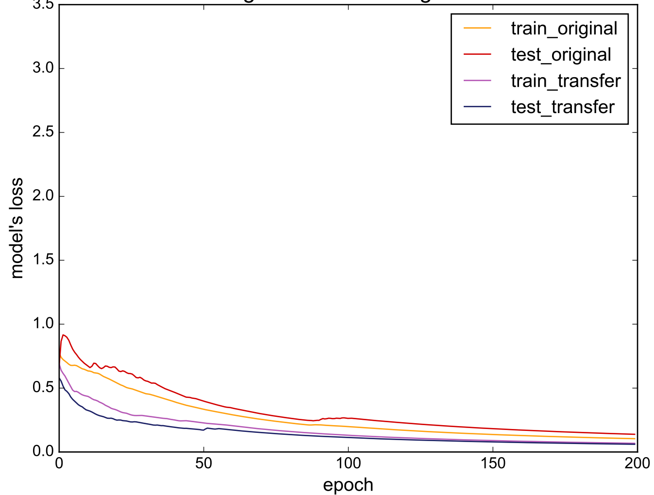
Source: ToeSegmentation2 - Target: TwoLeadECG
