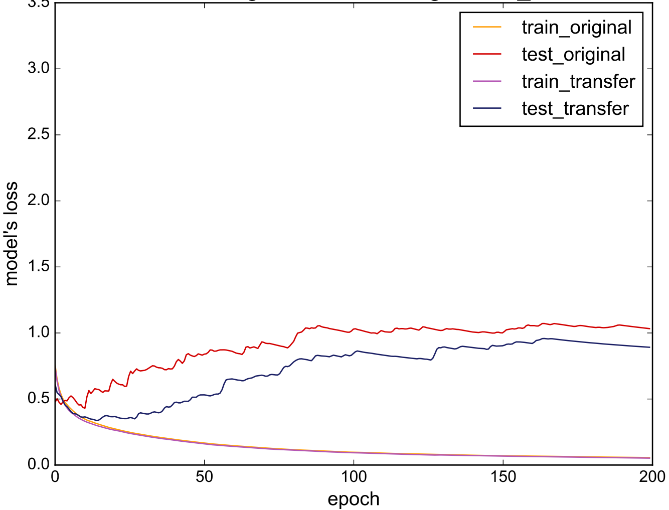
Source: ToeSegmentation2 - Target: Two_Patterns
