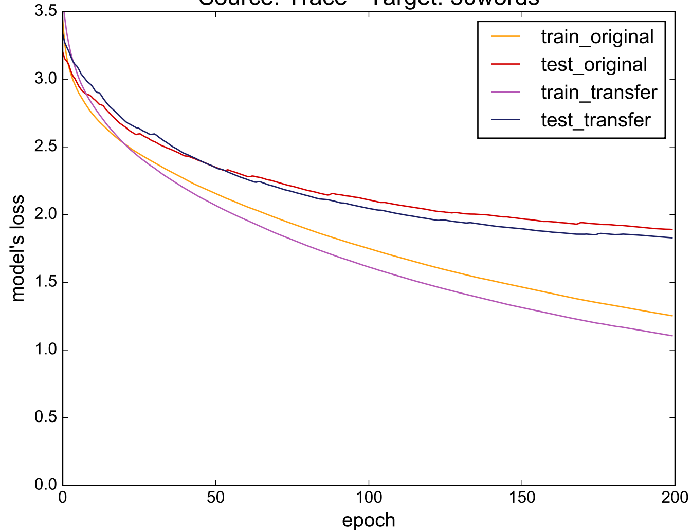
Source: Trace - Target: 50words
