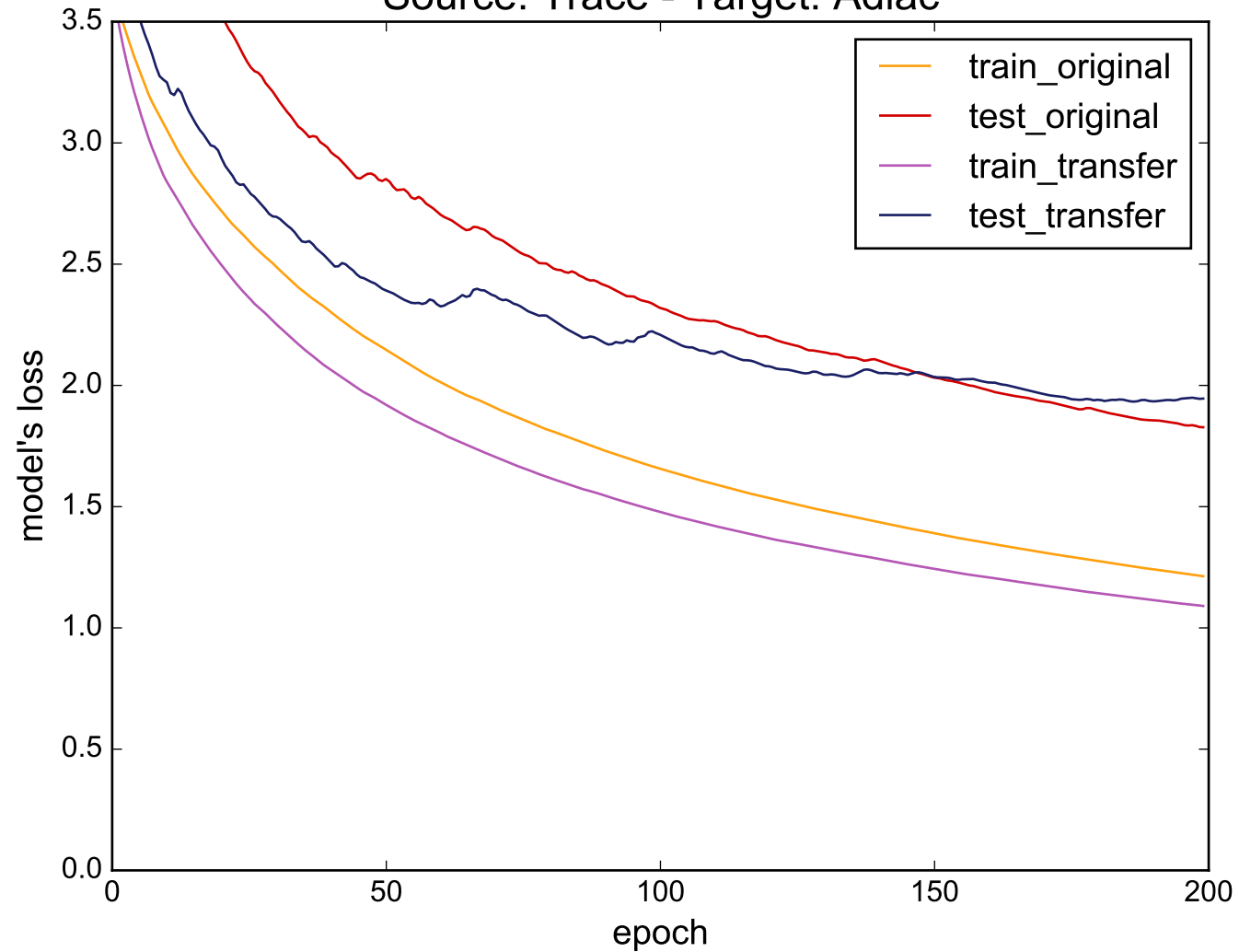
Source: Trace - Target: Adiac
