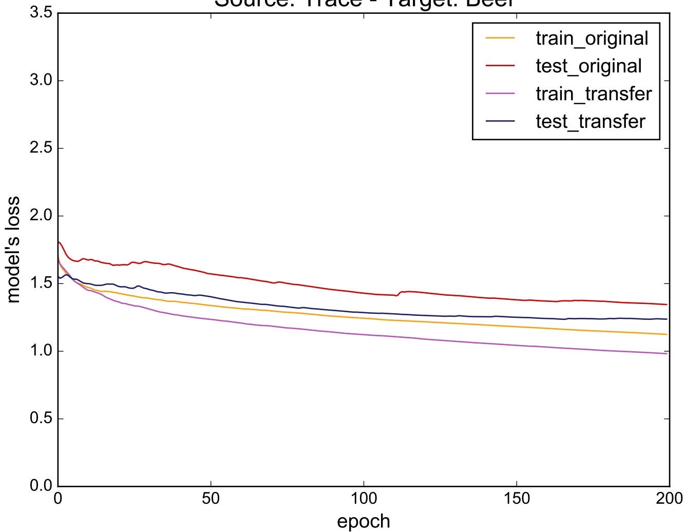
Source: Trace - Target: Beef
