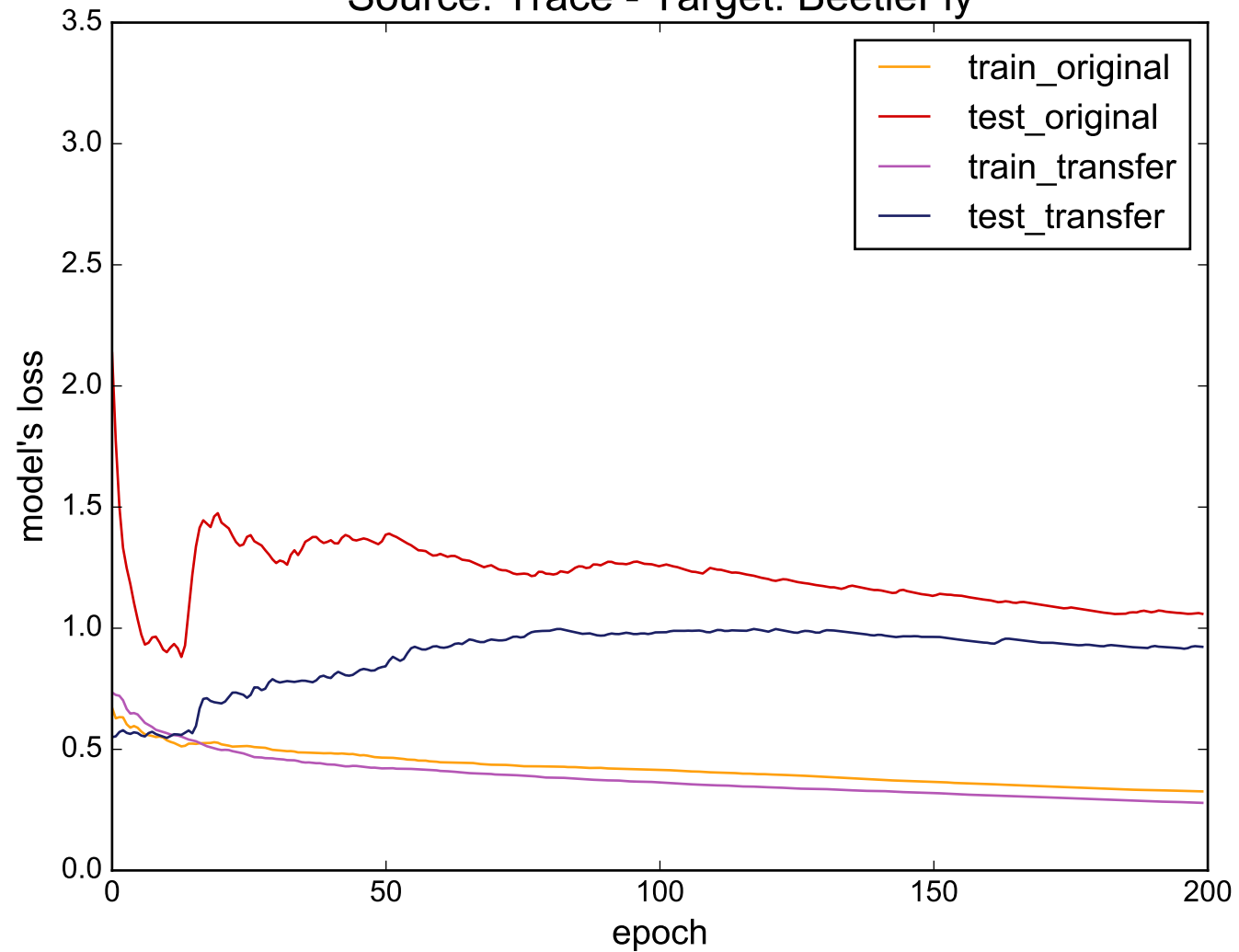
Source: Trace - Target: BeetleFly
