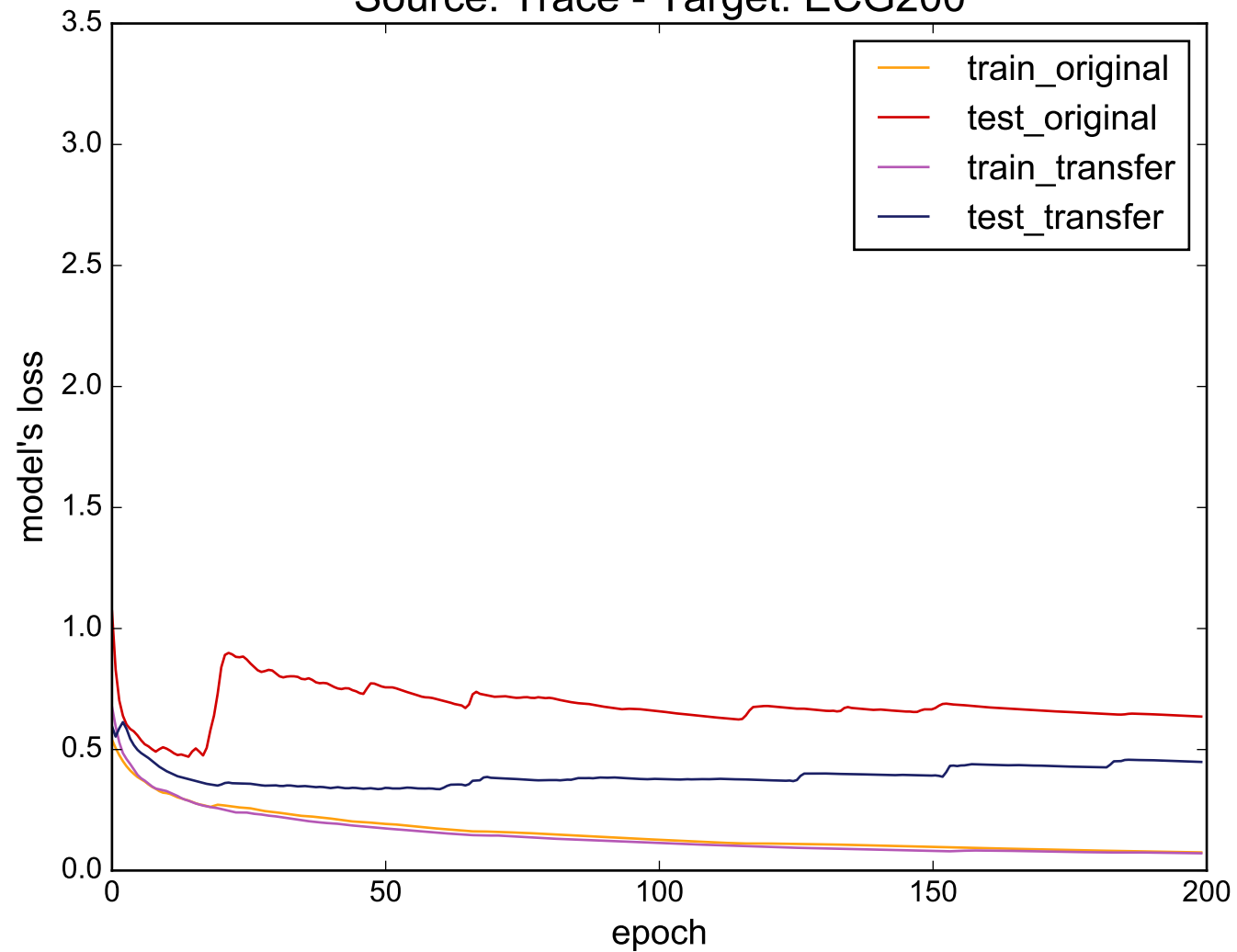
Source: Trace - Target: ECG200
