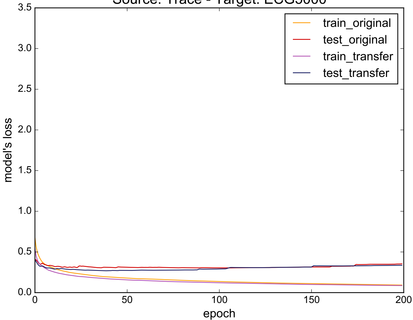
Source: Trace - Target: ECG5000
