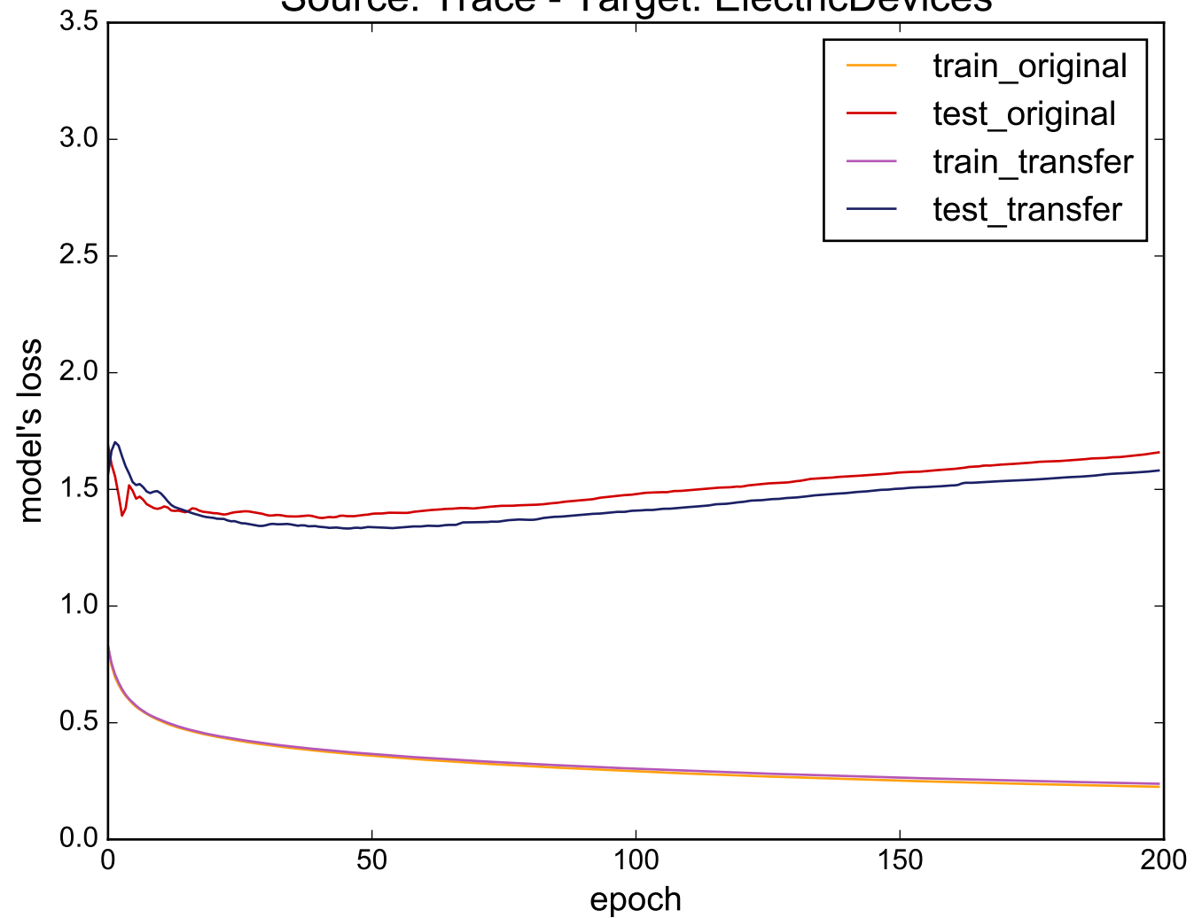
Source: Trace - Target: ElectricDevices
