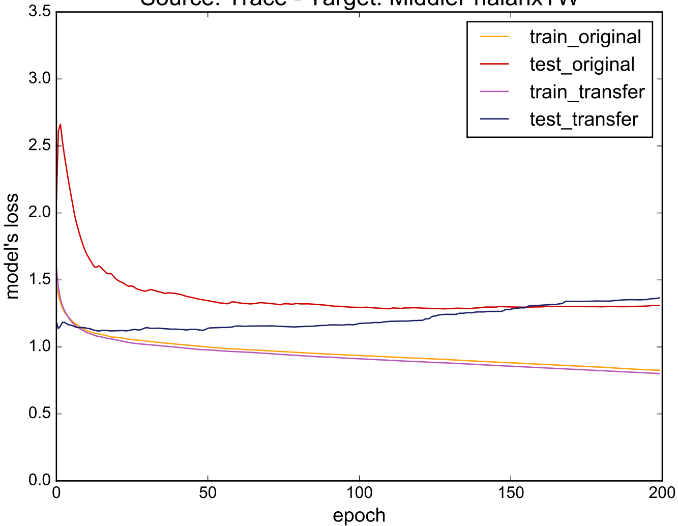
Source: Trace - Target: MiddlePhalanxTW
