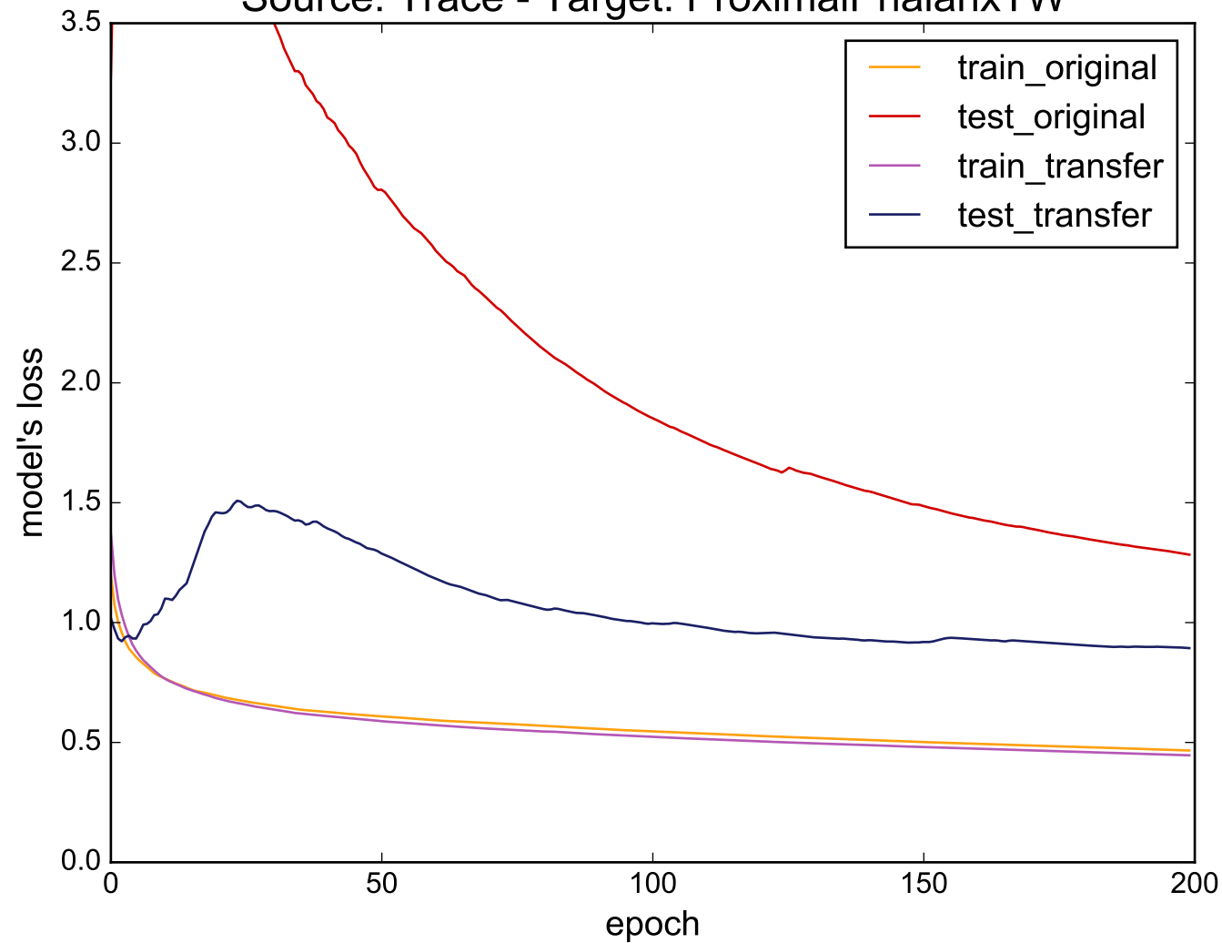
Source: Trace - Target: ProximalPhalanxTW
