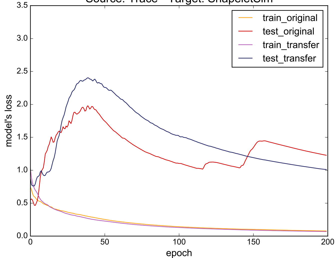
Source: Trace - Target: ShapeletSim
