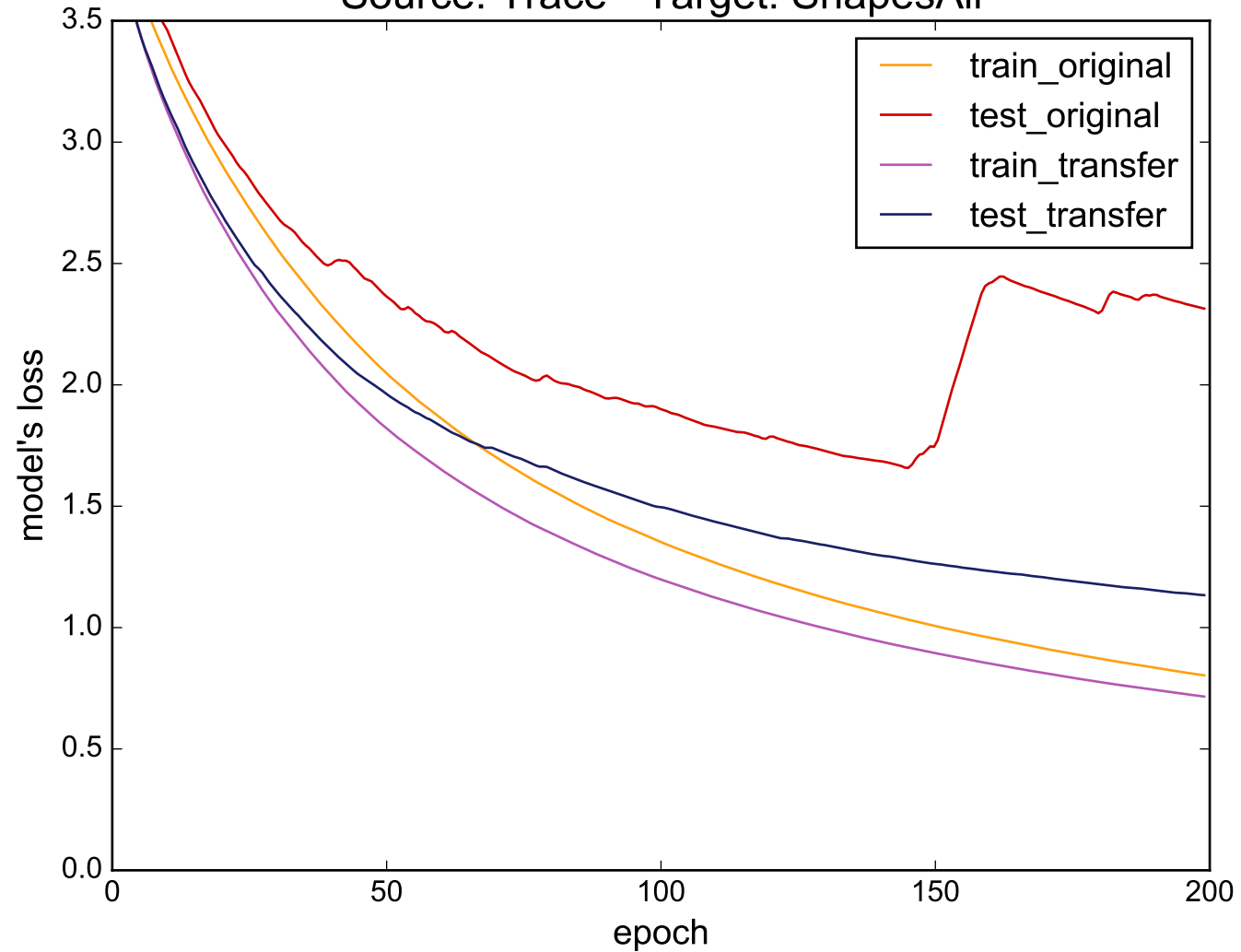
Source: Trace - Target: ShapesAll
