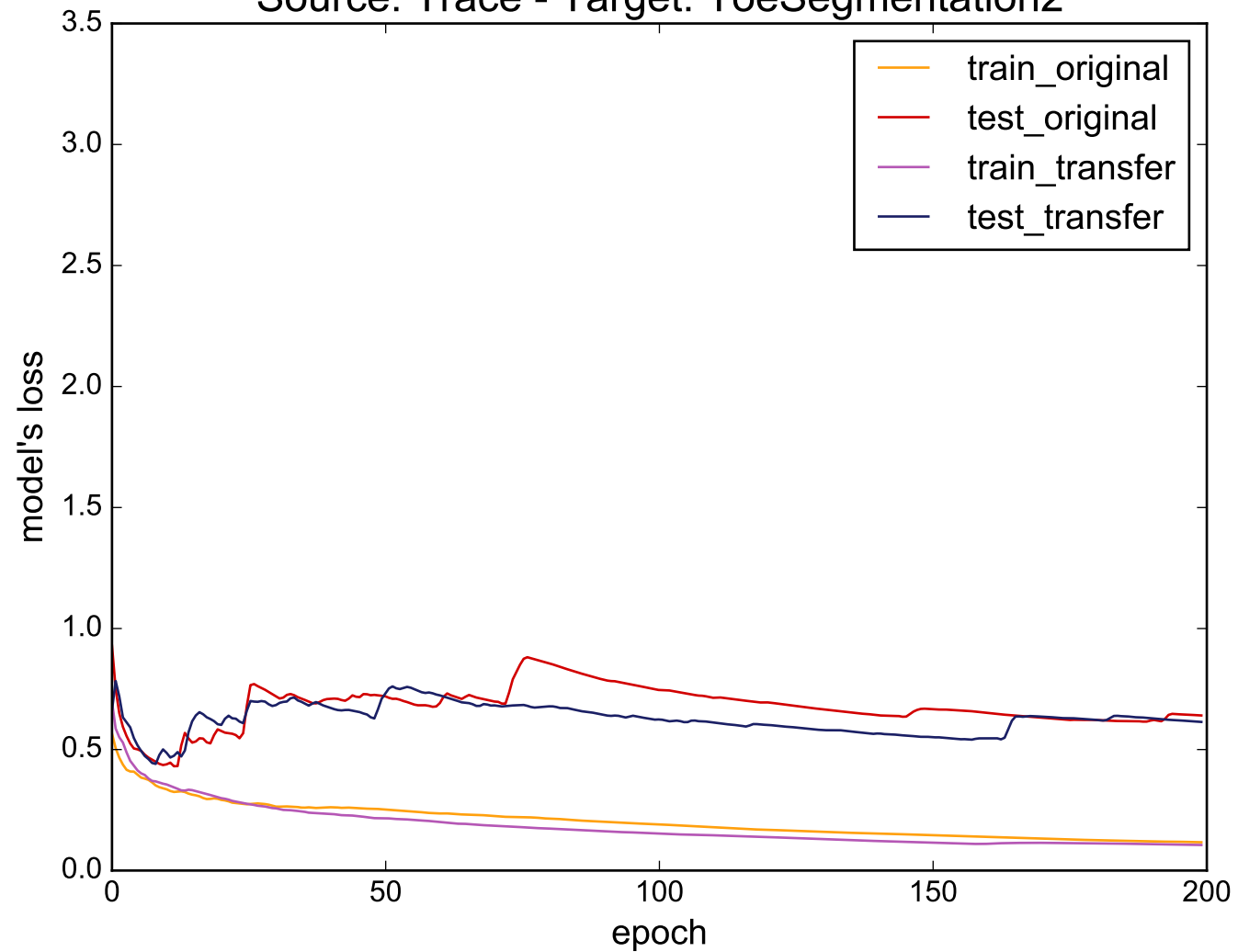
Source: Trace - Target: ToeSegmentation2
