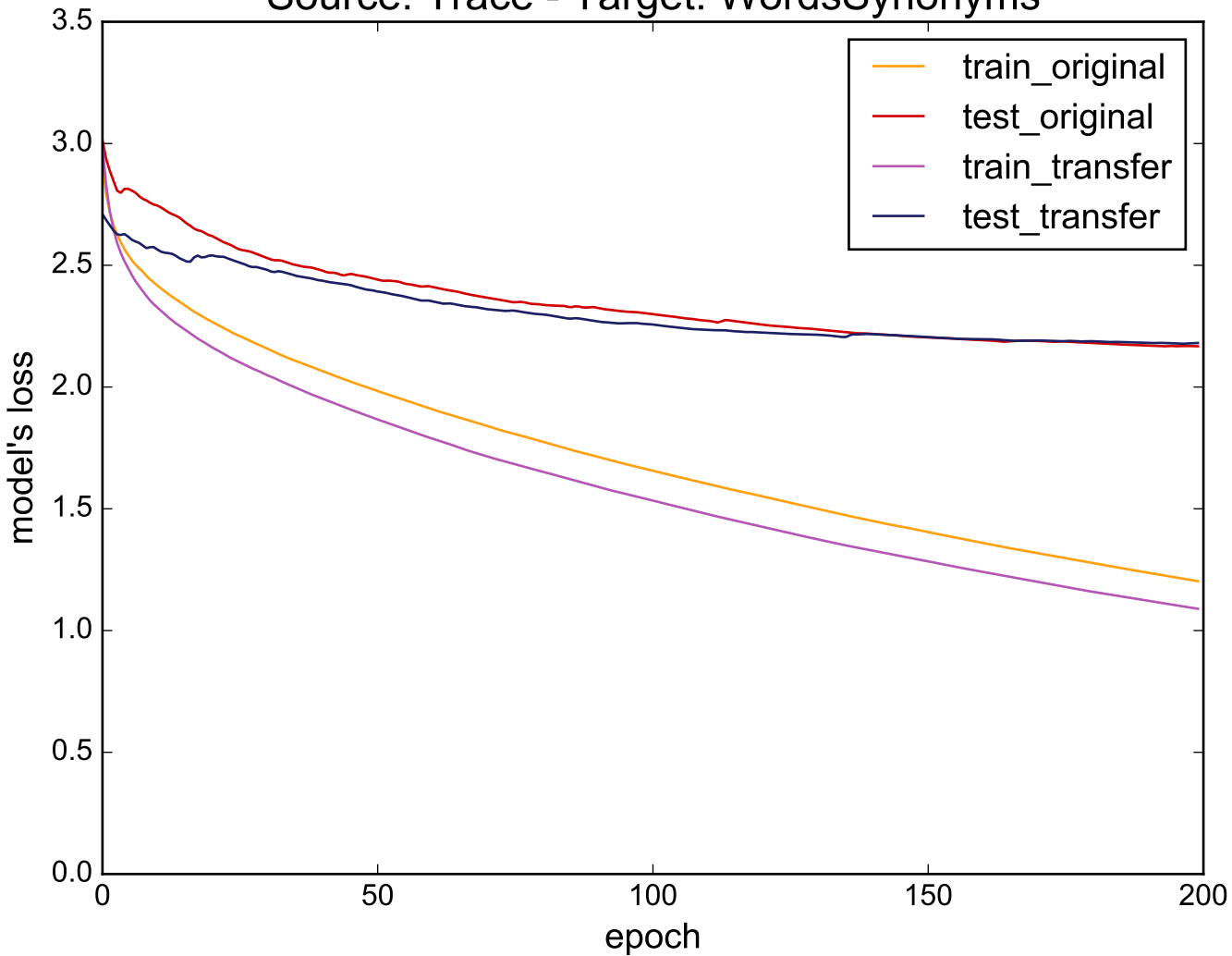
Source: Trace - Target: WordsSynonyms
