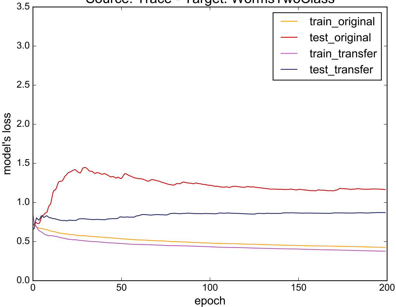
Source: Trace - Target: WormsTwoClass
