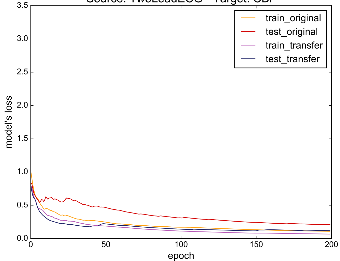
Source: TwoLeadECG - Target: CBF
