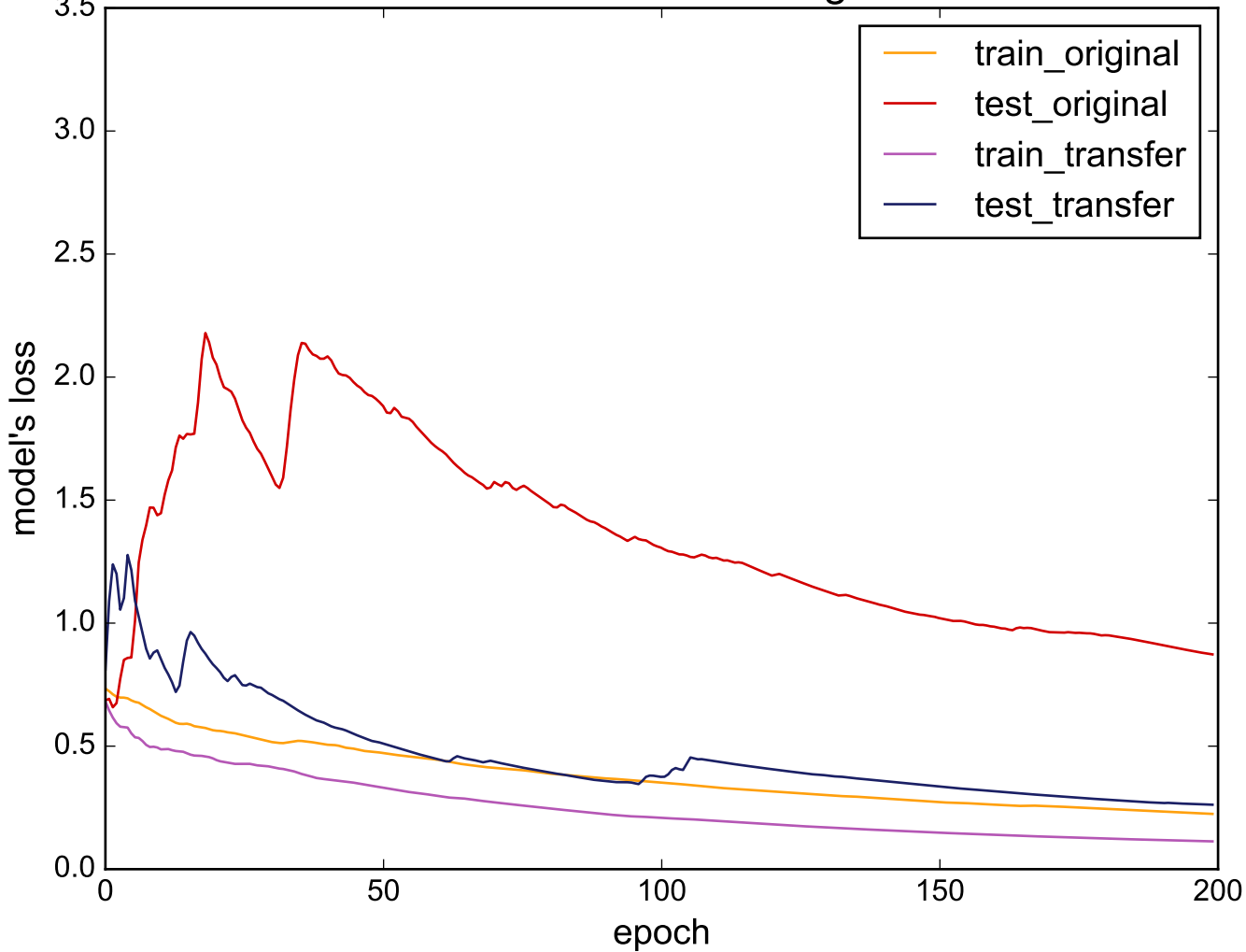
Source: TwoLeadECG - Target: Coffee
