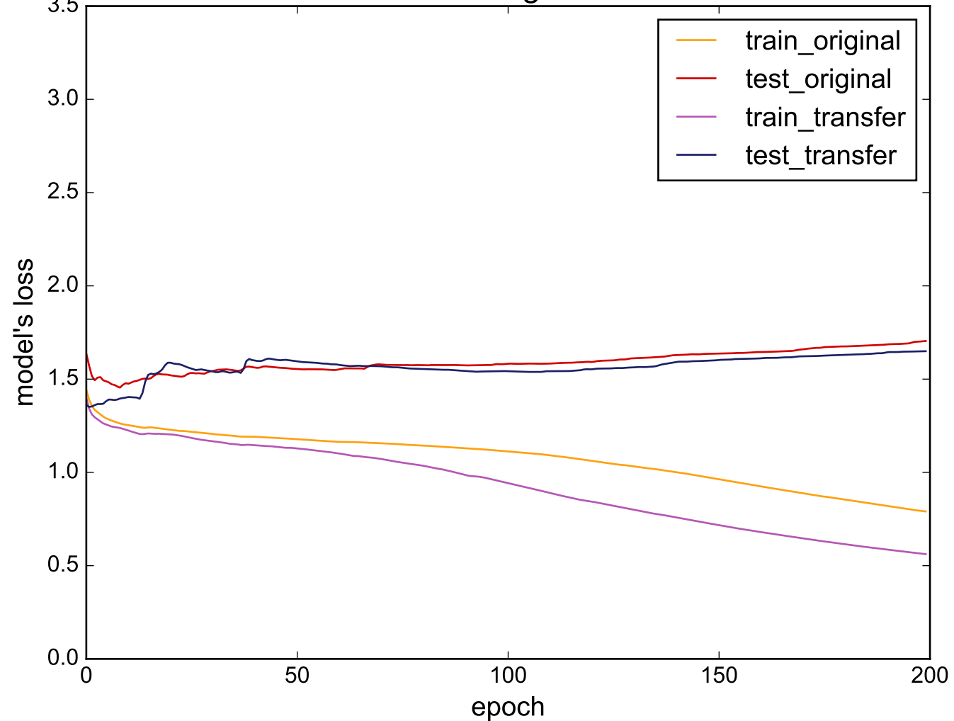
Source: TwoLeadECG - Target: DiatomSizeReduction
