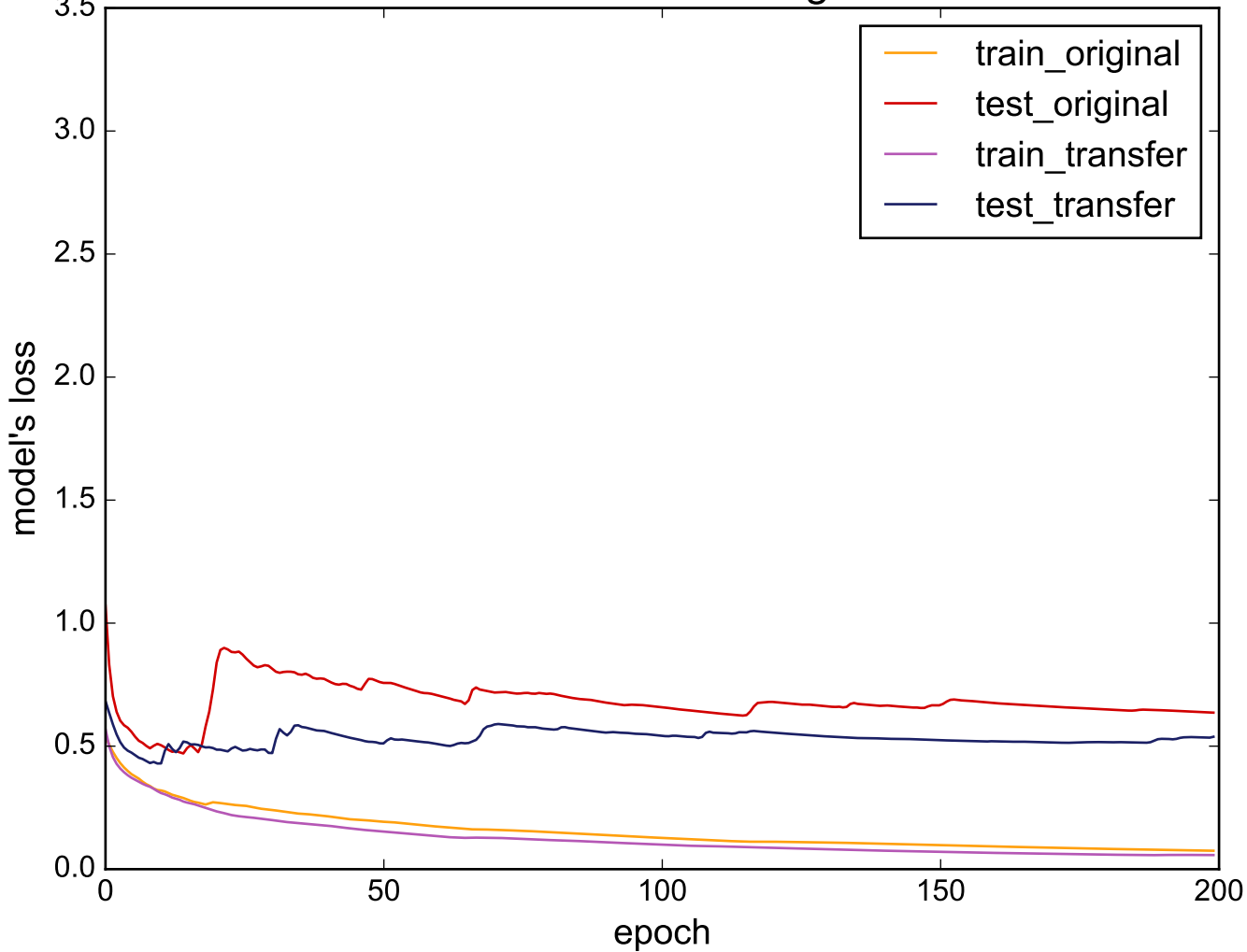
Source: TwoLeadECG - Target: ECG200
