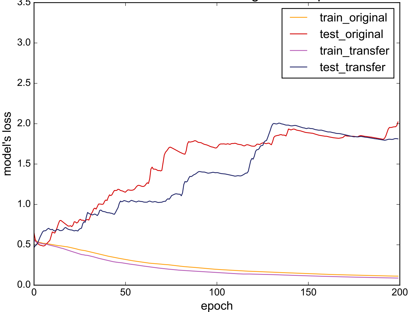
Source: TwoLeadECG - Target: Earthquakes
