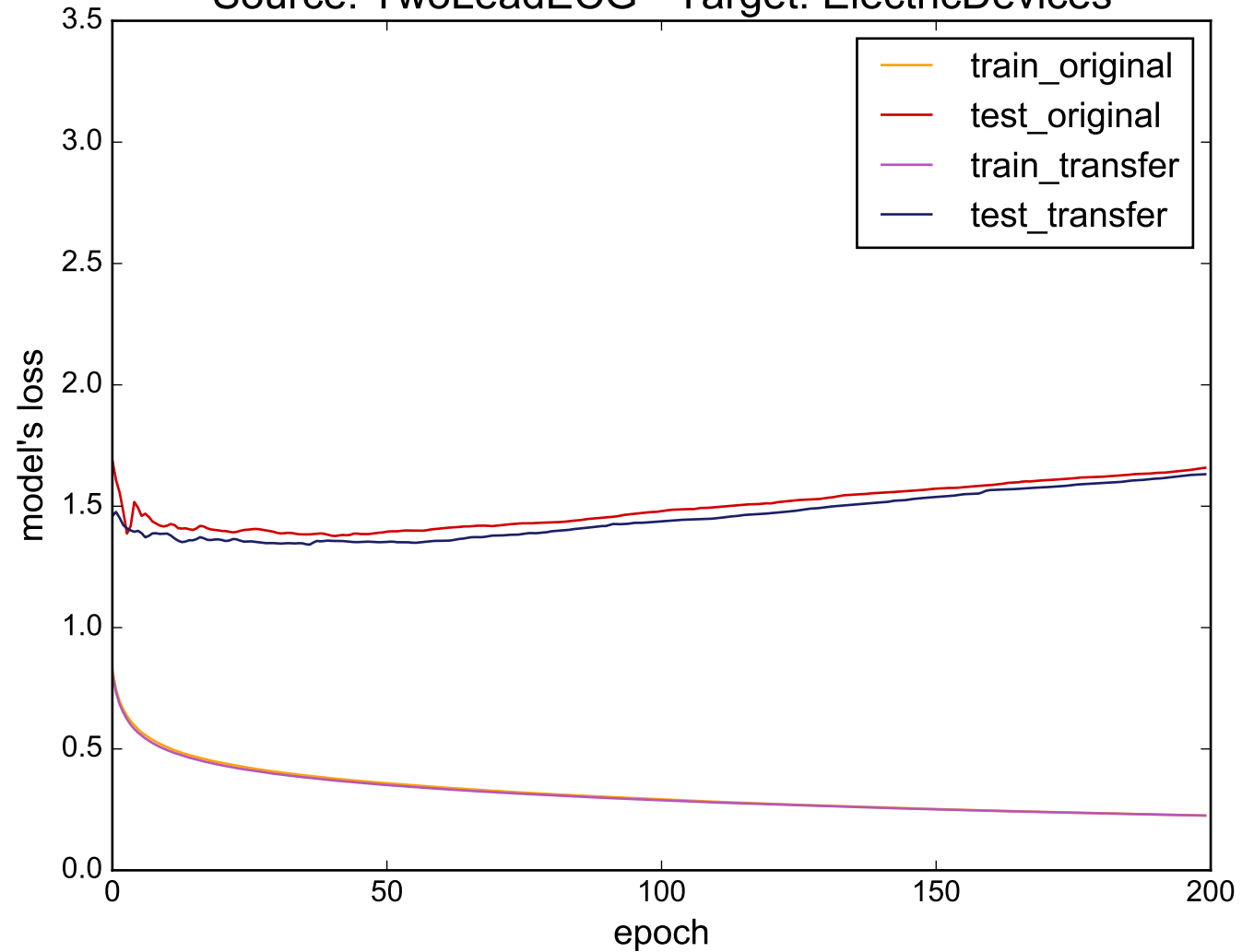
Source: TwoLeadECG - Target: ElectricDevices
