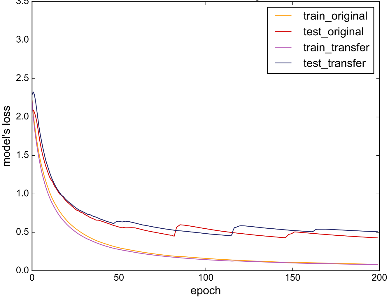
Source: TwoLeadECG - Target: FaceAll
