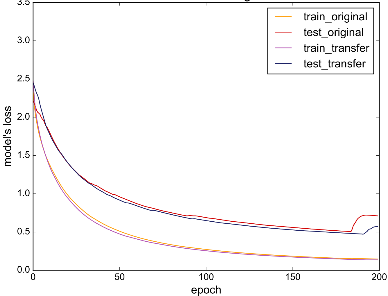
Source: TwoLeadECG - Target: FacesUCR
