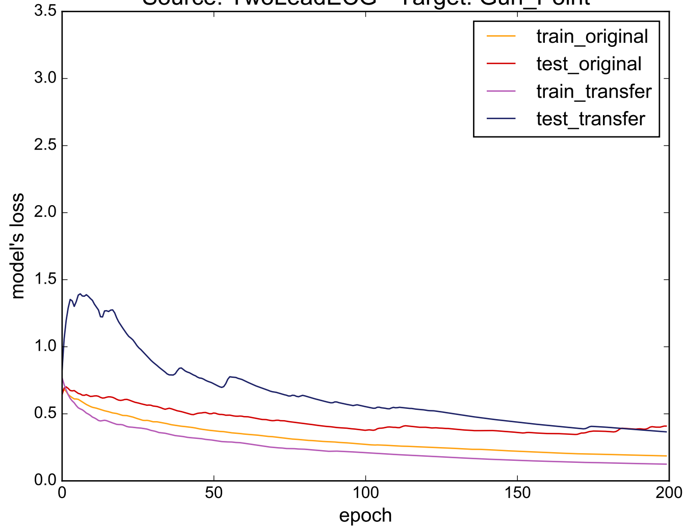
Source: TwoLeadECG - Target: Gun_Point
