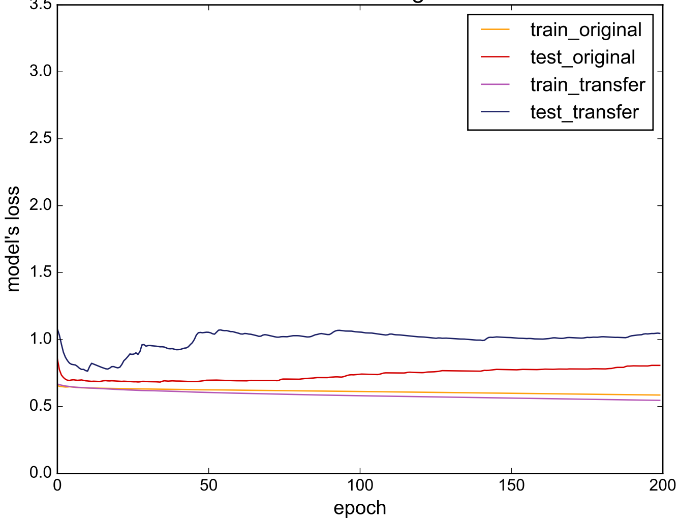
Source: TwoLeadECG - Target: HandOutlines
