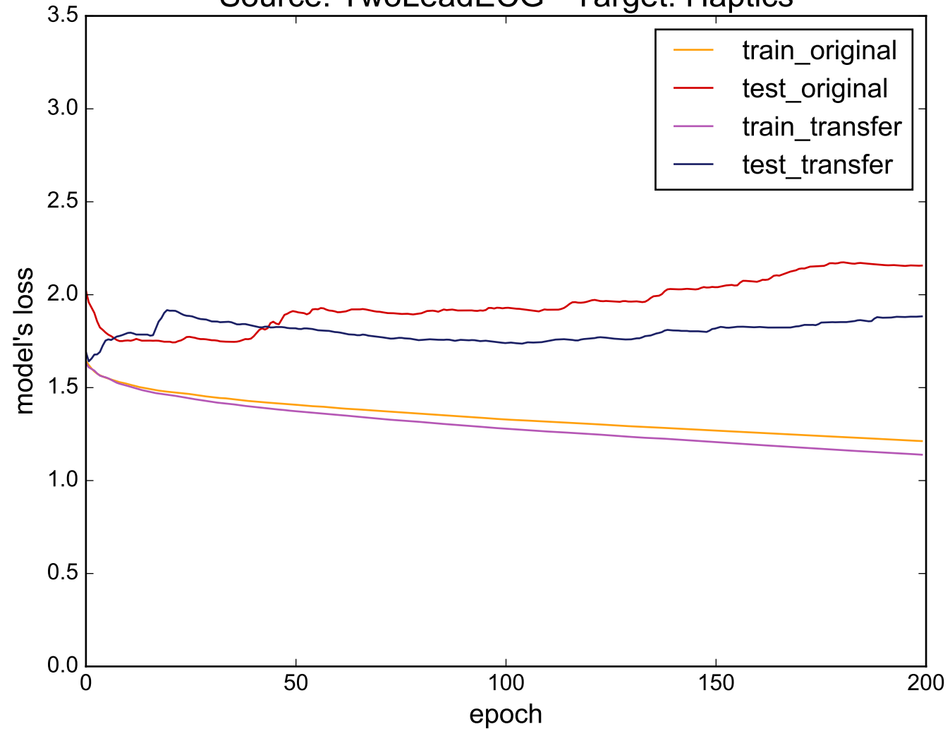
Source: TwoLeadECG - Target: Haptics
