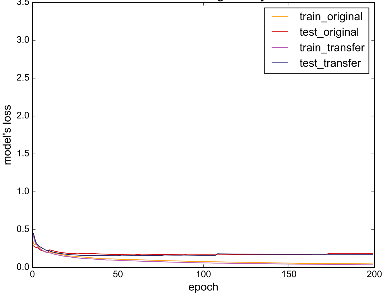
Source: TwoLeadECG - Target: ItalyPowerDemand
