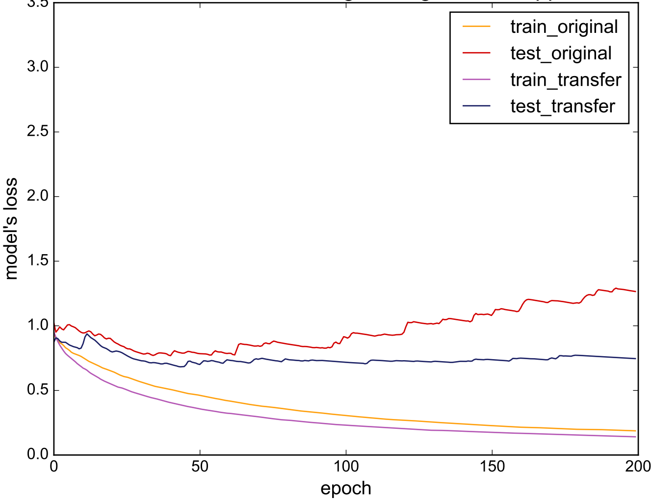
Source: TwoLeadECG - Target: LargeKitchenAppliances
