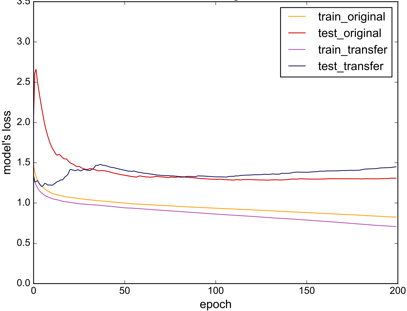
Source: TwoLeadECG - Target: MiddlePhalanxTW
