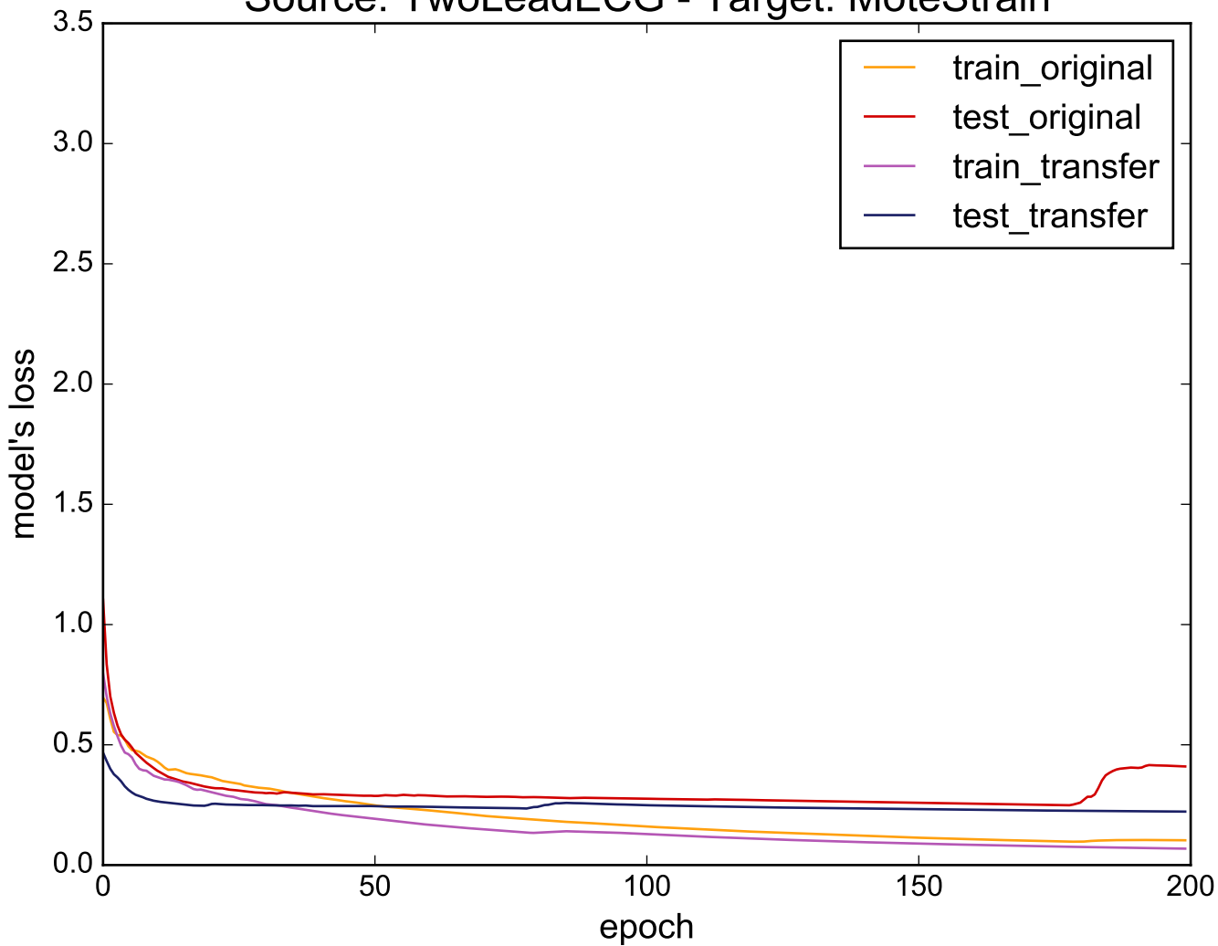
Source: TwoLeadECG - Target: MoteStrain
