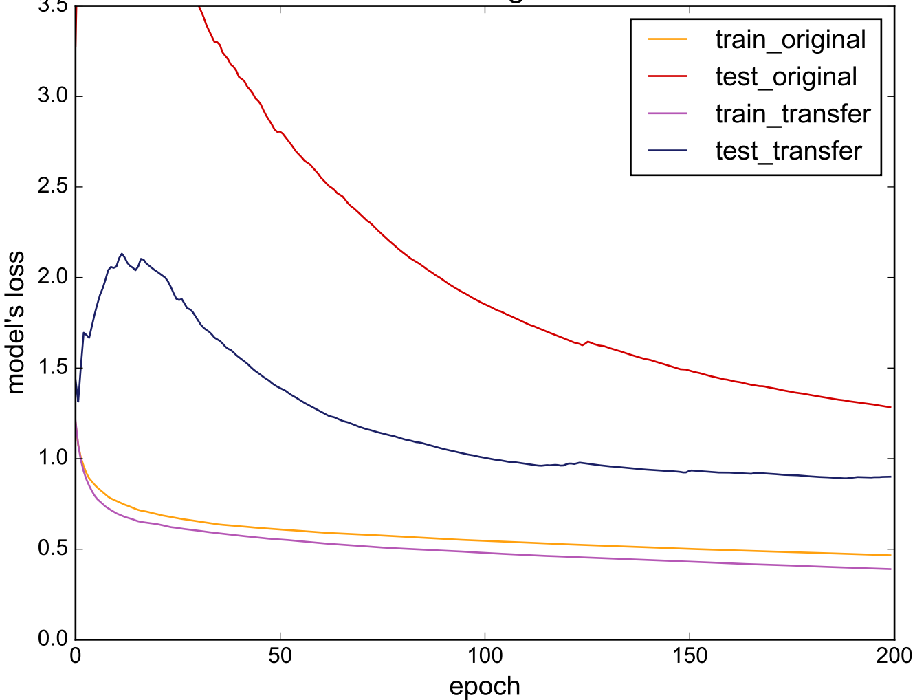
Source: TwoLeadECG - Target: ProximalPhalanxTW
