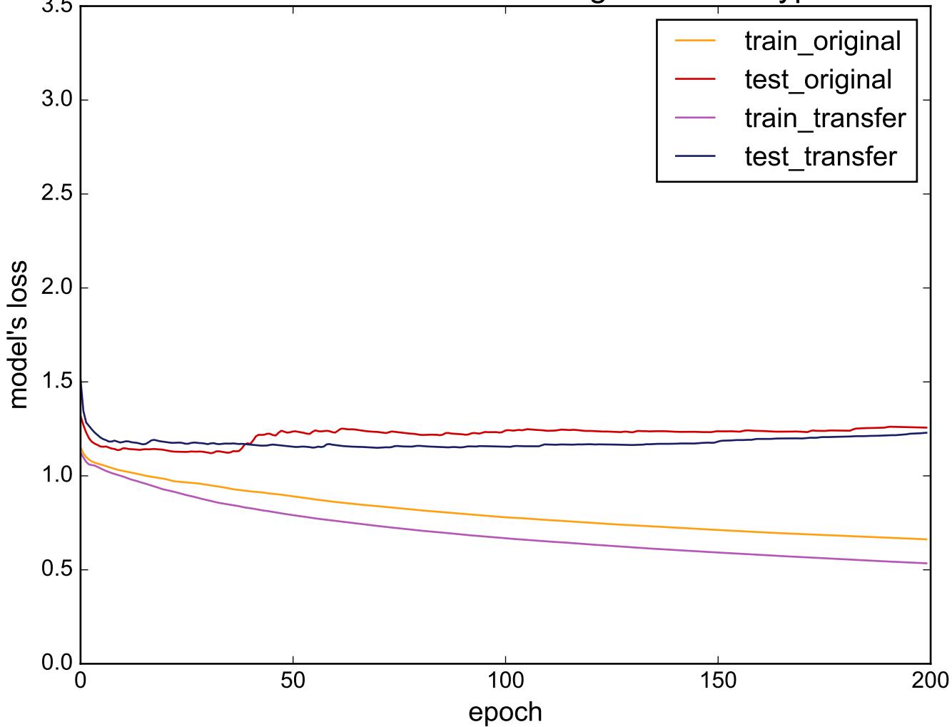
Source: TwoLeadECG - Target: ScreenType
